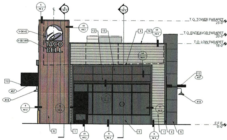
SOUTH ELEVATION 1/8" = 1'-0" C
