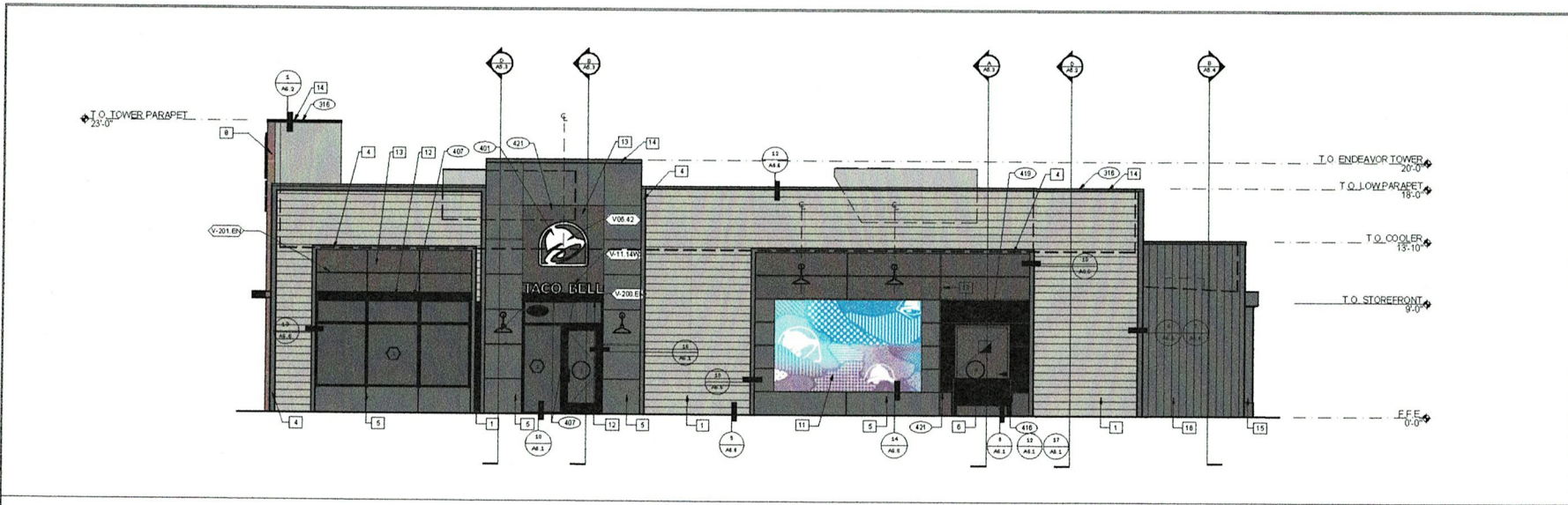
EAST ELEVATION 1/4" = 1'-0" A
